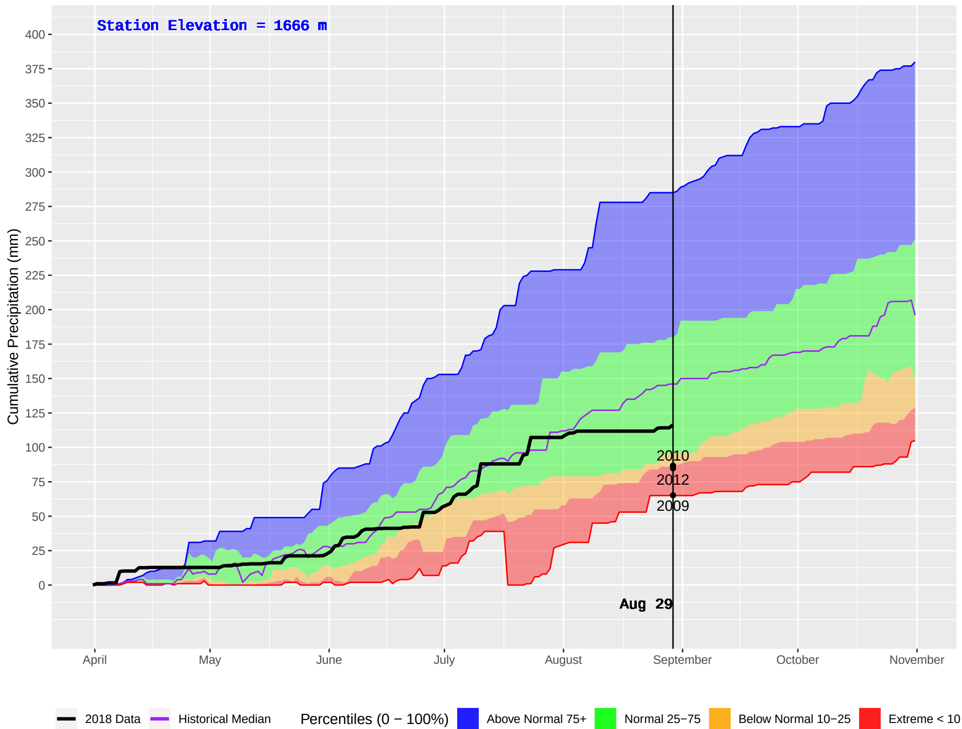
BALDFACE (221) : Historical (1992–2016) and Current (2018) Daily Cumulative Precipitation
